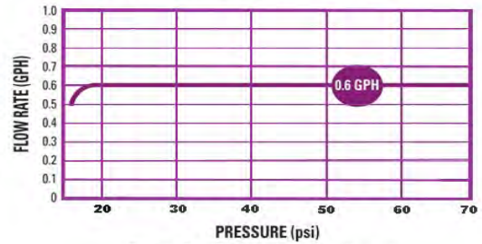
DRIPPER FLOW RATE VS. PRESSURE
