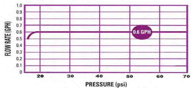
DRIPPER FLOW RATE VS. PRESSURE
